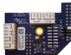
AND-STROBE-KIT-1 includes AND-PIA-2
