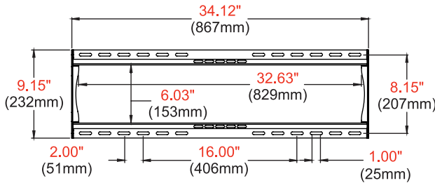
WALL PLATE
