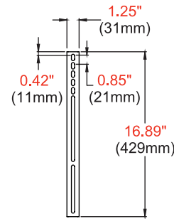
VERTICAL ADAPTOR
