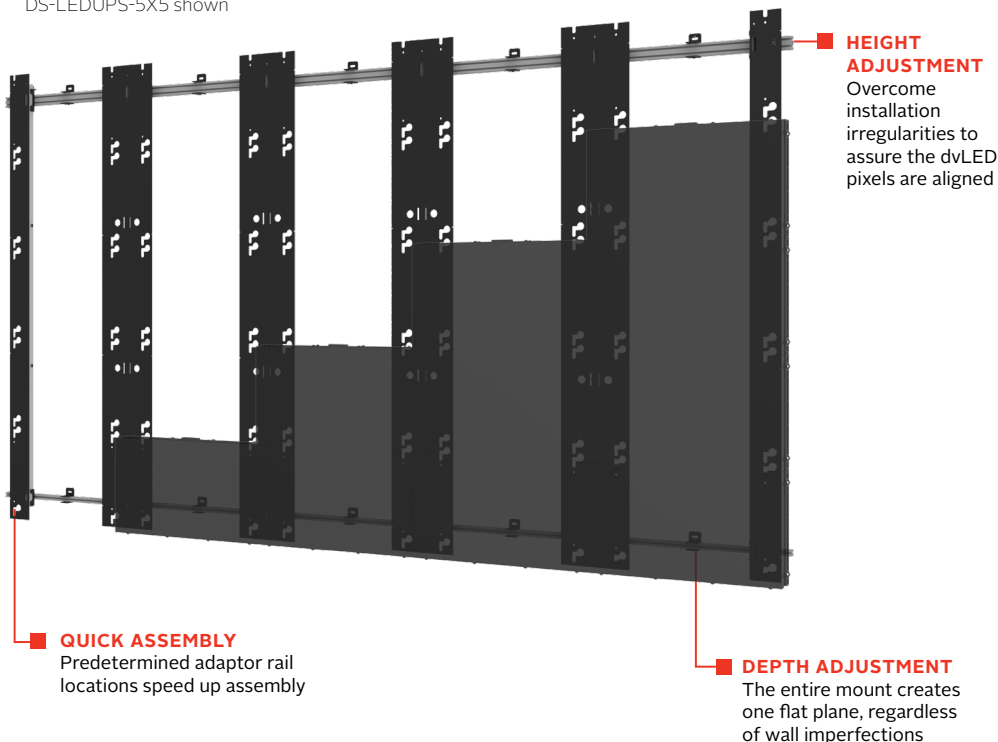
DS-LEDUPS-5X5 shown
