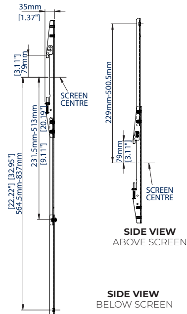
MOUNTING ON A BT9903
