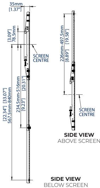
MOUNTING ON A BT8431 / BT8432 / BT8441 / BT8442
