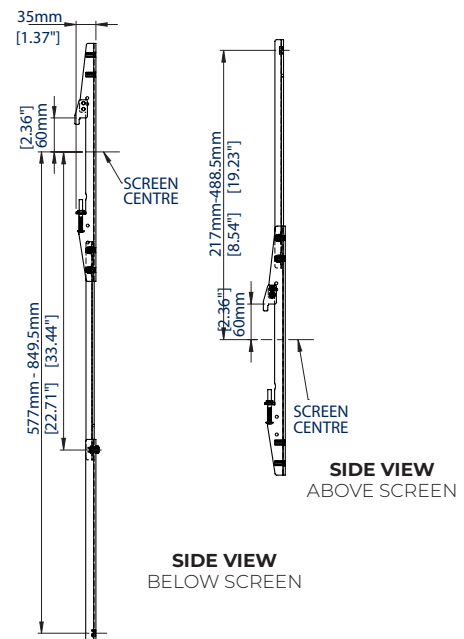
MOUNTING ON A BT8390 RAIL
