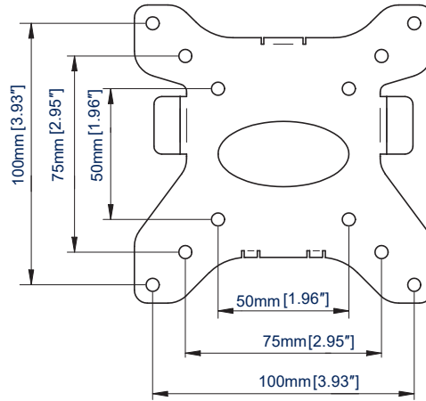
FRONT VIEW INTERFACE PLATE
