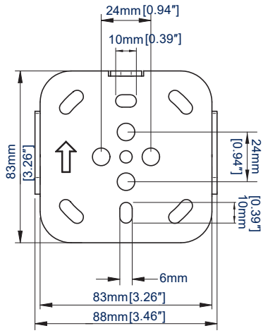
FRONT VIEW WALL PLATE
