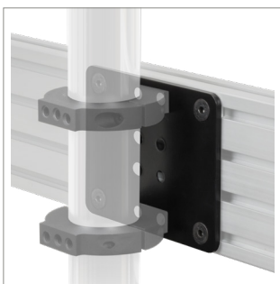
Mounts BT8390 rails to System 2 BT7850 poles using accessory collars
