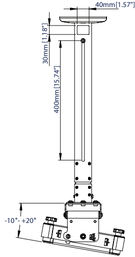
SIDE VIEW WITH INTERFACE TILT
