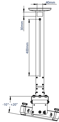
SIDE VIEW WITH INTERFACE TILT
