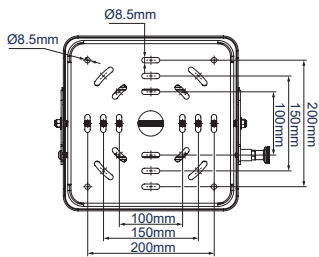
BOTTOM VIEW / INTERFACE PLATE
