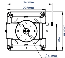
TOP VIEW WITH CEILING PLATE
