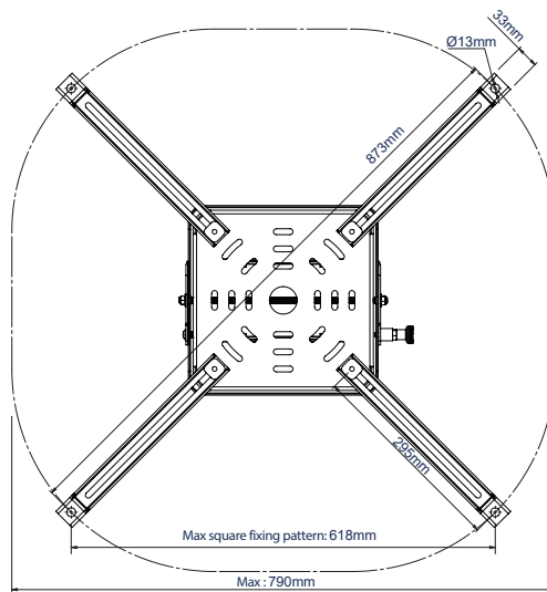
INTERFACE WITH LONG EXTENSION LEGS & SHORT EXTENSION LEGS
