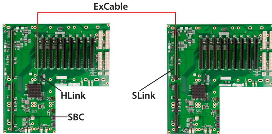
System providing up to 17 PCI Express slots
