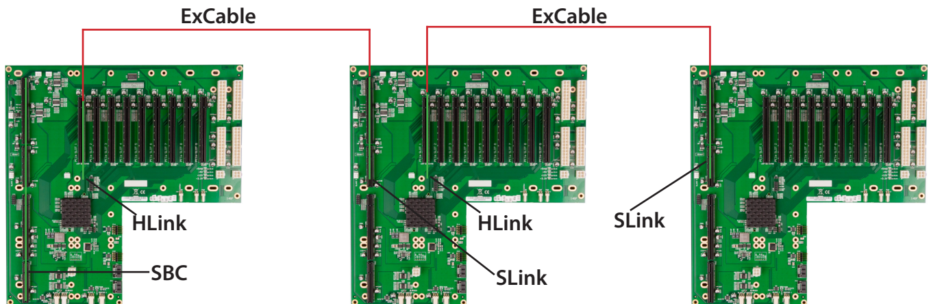
System providing up to 25 PCI Express slots
